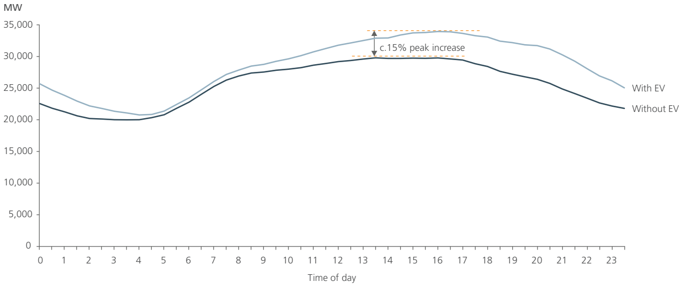
Figure 3 EV impact on the Australian electricity network (50% EV adoption) 6
